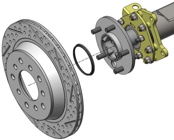
Figure 6a – Rotor and Centering Ring Installation
