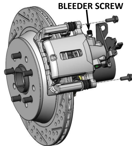
Figure 9b - Caliper Installation and Bleeder Screw Orientation
