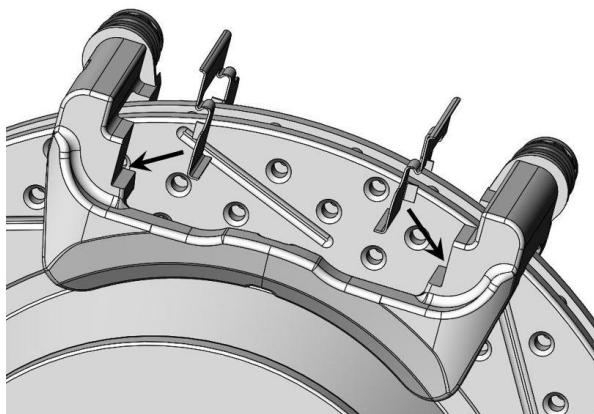
Figure 8a– Abutment Clips Installation
