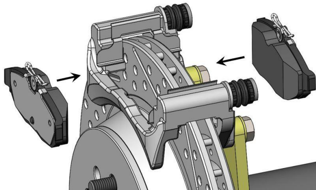
Figure 9a – Brake Pad Installation
