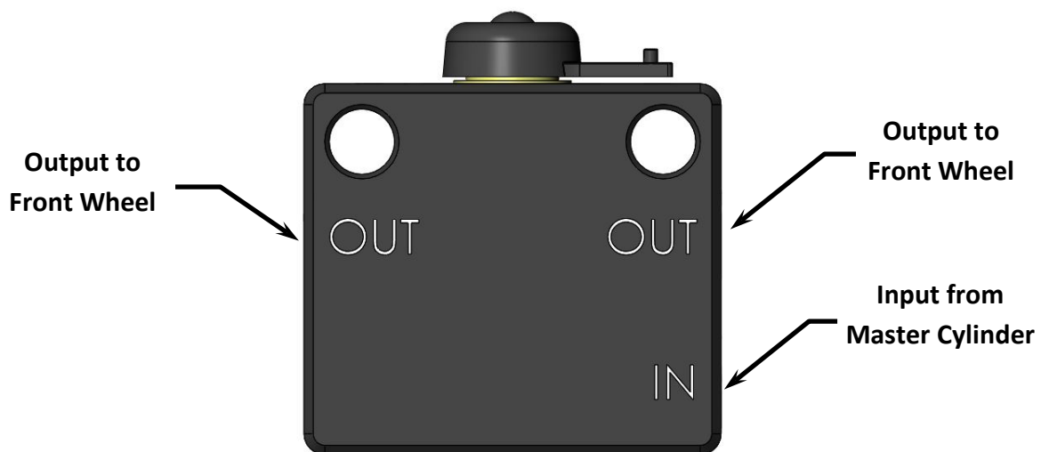
Figure 1 – Port Locations
