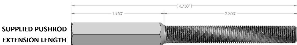
Figure 1 – Pushrod Extension
